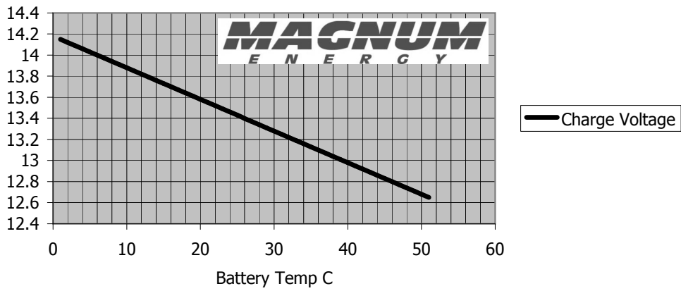
Temperature compensation for AGM in float charge mode (30mv per degC per UL1776)
