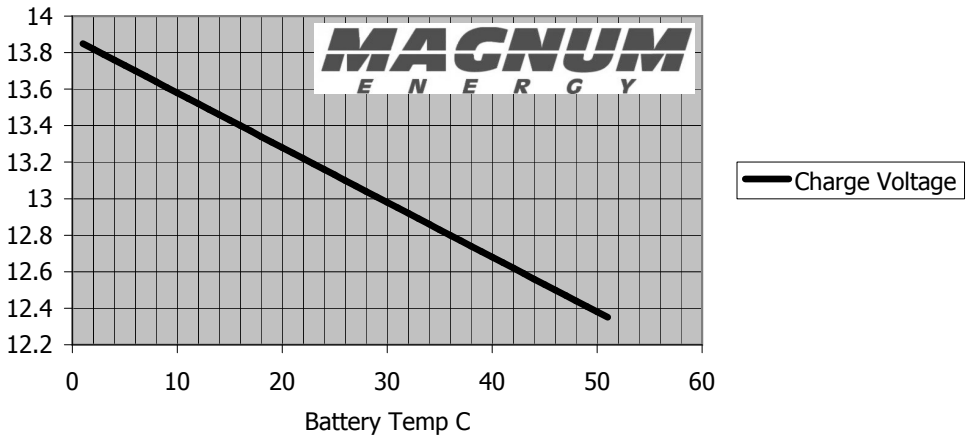
Temperature compensation for AGM in float charge mode (30mv per degC per UL1776)
