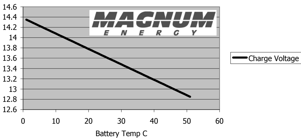
Temperature compensation for Gel in float charge mode (30mv per degC per UL1776)
